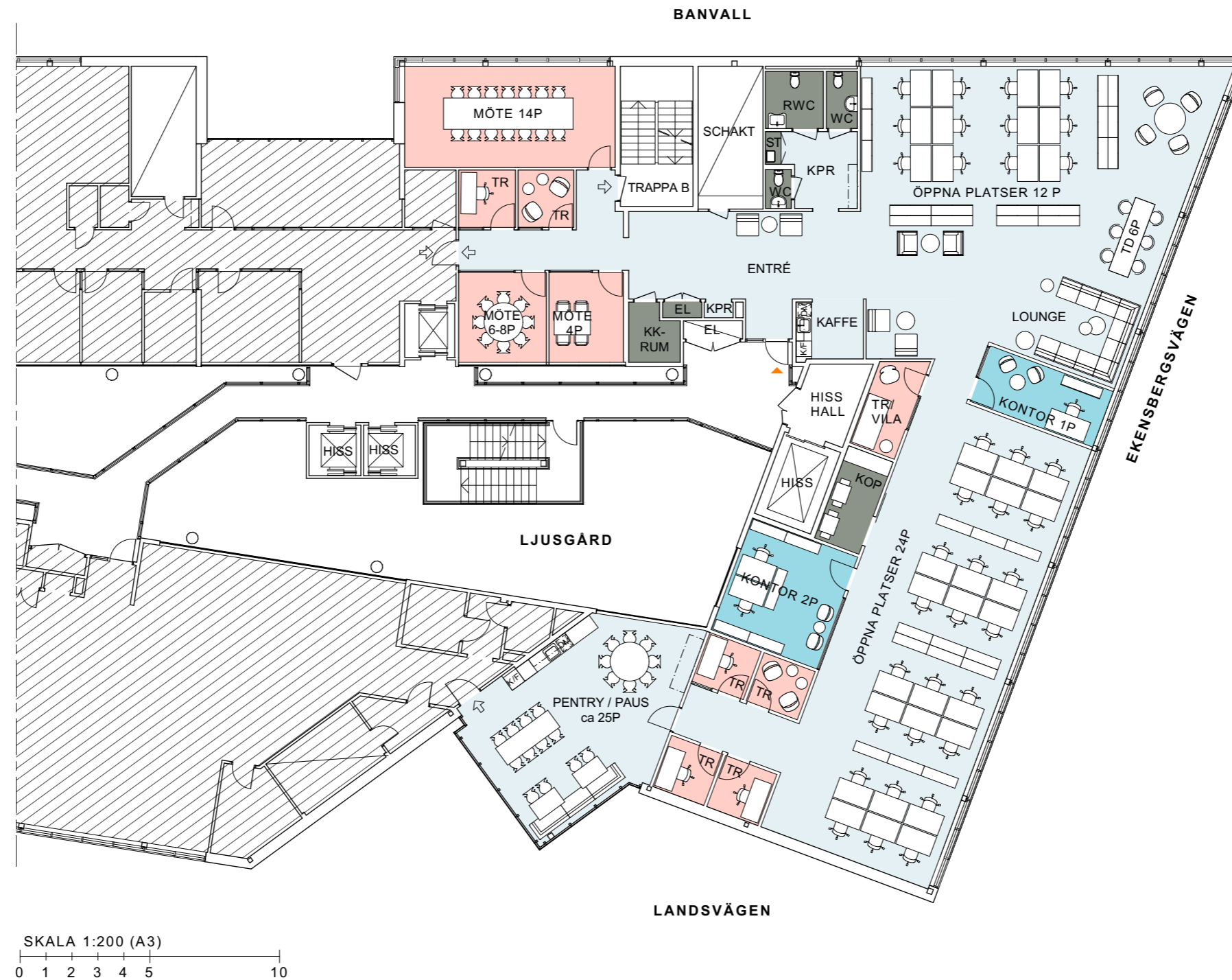
ORIENTERINGSPLAN
