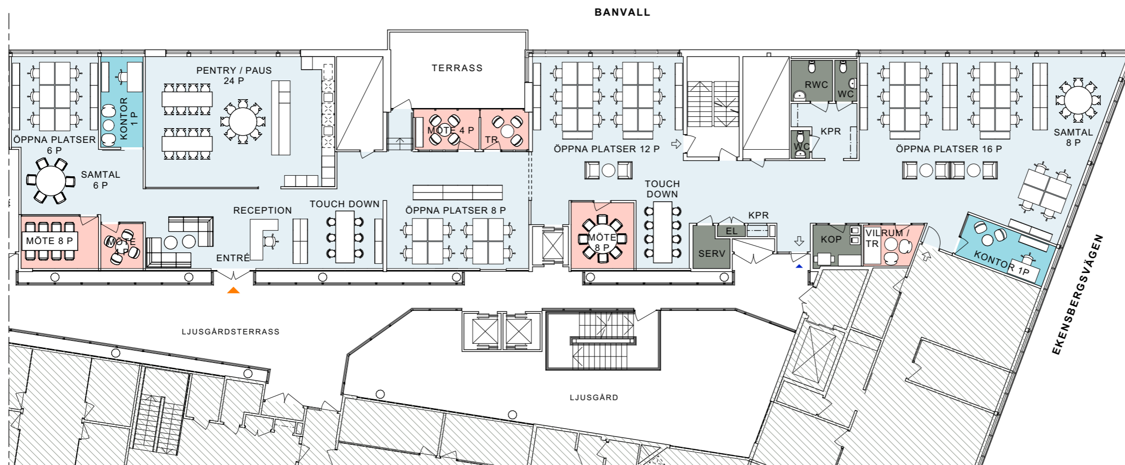
ORIENTERINGSPLAN
